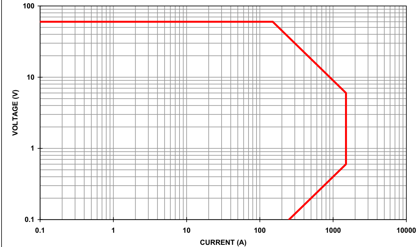
PLW9K-60-1500 (60V,1500A,9KW) OPERATIONAL CURVE
