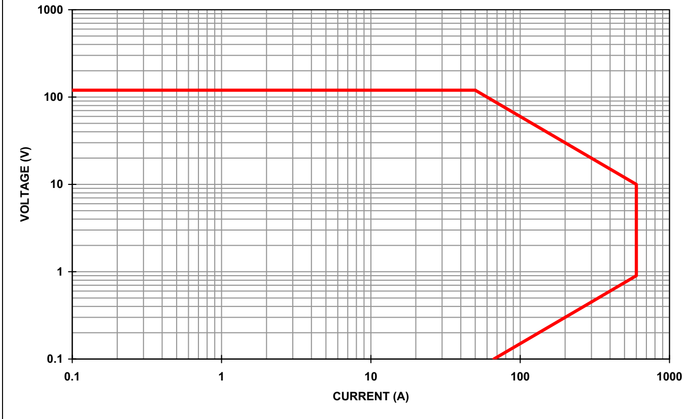
PLW6K-120-600 (120V,600A,6KW) OPERATIONAL CURVE
