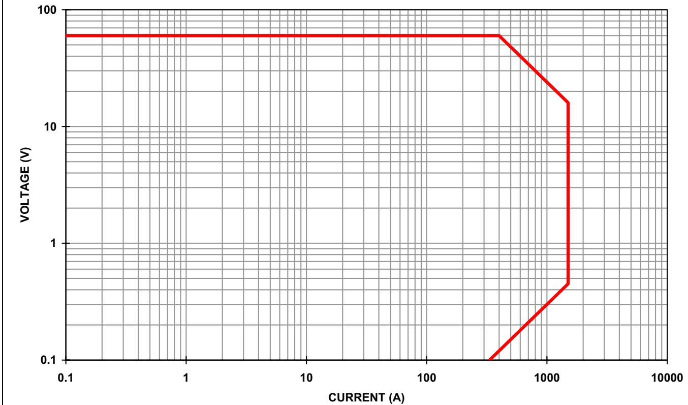
PLW24K-60-1500 (60V,1500A,24KW) OPERATIONAL CURVE
