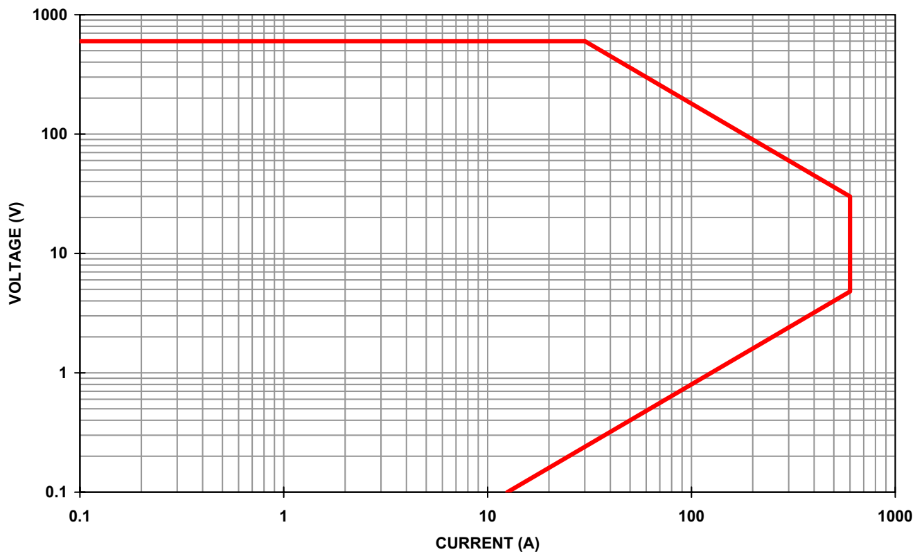
PLW18K-600-600 (600V,600A,18KW) OPERATIONAL CURVE
