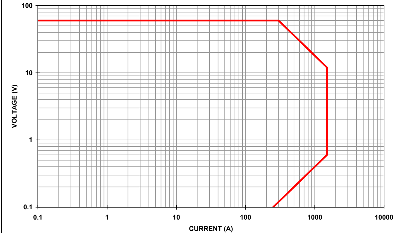
PLW18K-60-1500 (60V,1500A,18KW) OPERATIONAL CURVE
