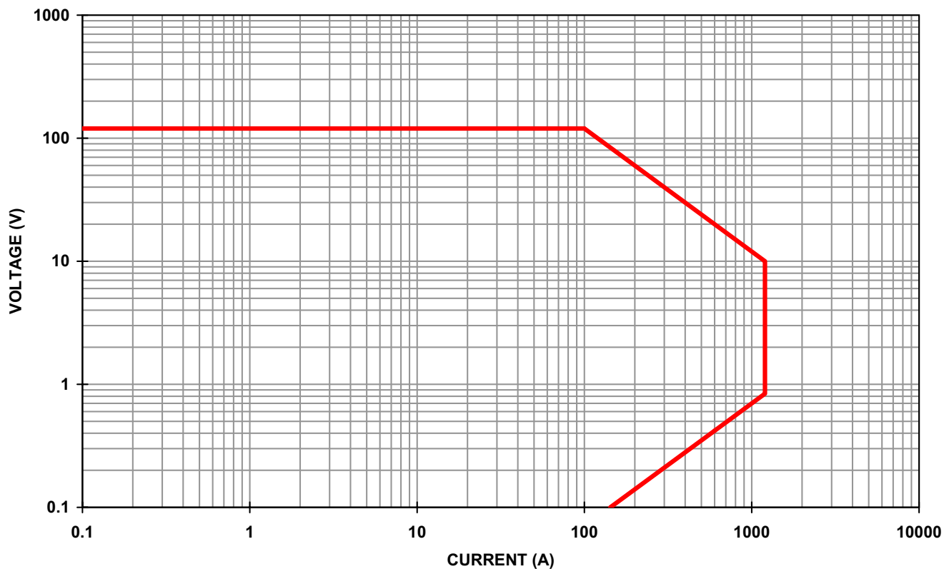
PLW12K-120-1200 (120V,1200A,12KW) OPERATIONAL CURVE
