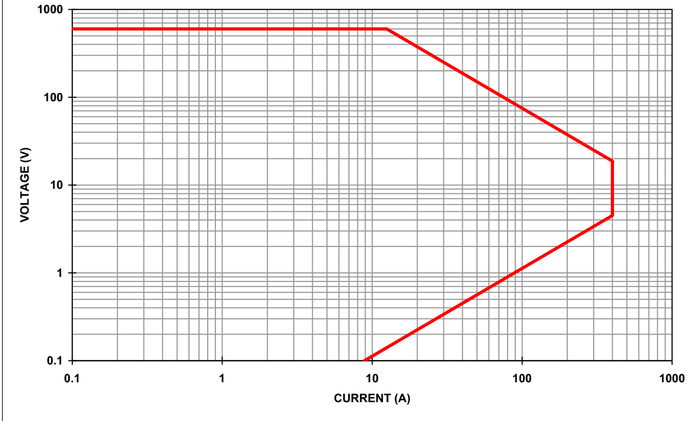
PLA7.5K-600-400 (600V,400A,7.5KW) OPERATIONAL CURVE
