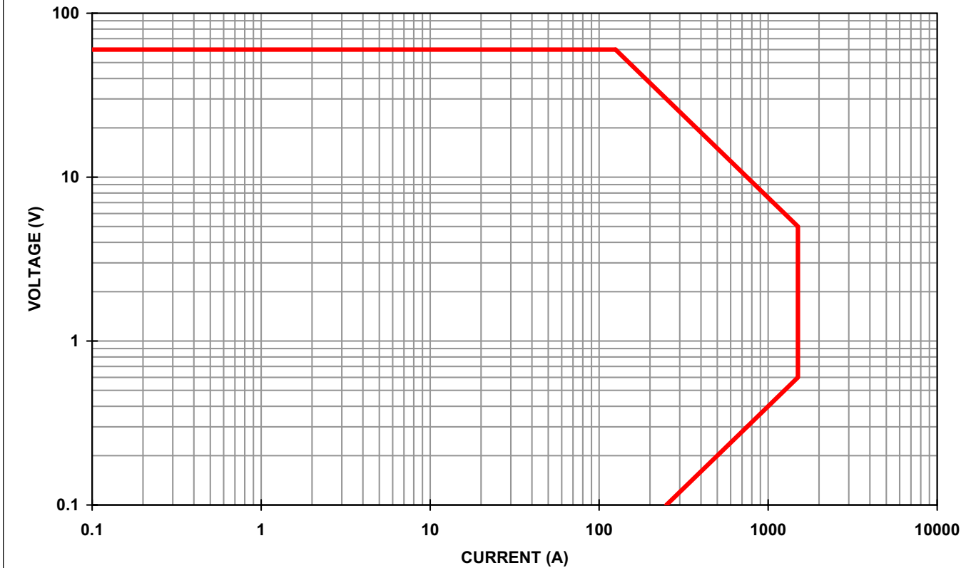
PLA7.5K-60-1500 (60V,1500A,7.5KW) OPERATIONAL CURVE
