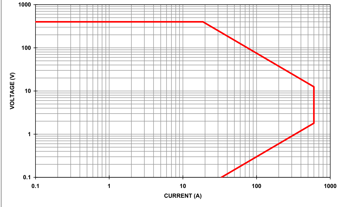
PLA7.5K-400-600 (400V,600A,7.5KW) OPERATIONAL CURVE
