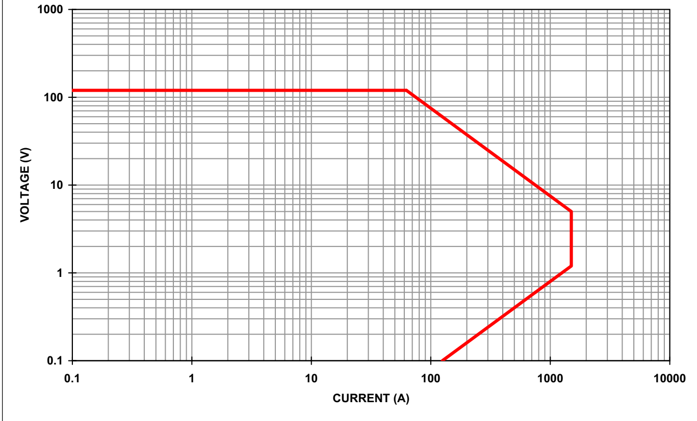
PLA7.5K-120-1500 (120V,1500A,7.5KW) OPERATIONAL CURVE
