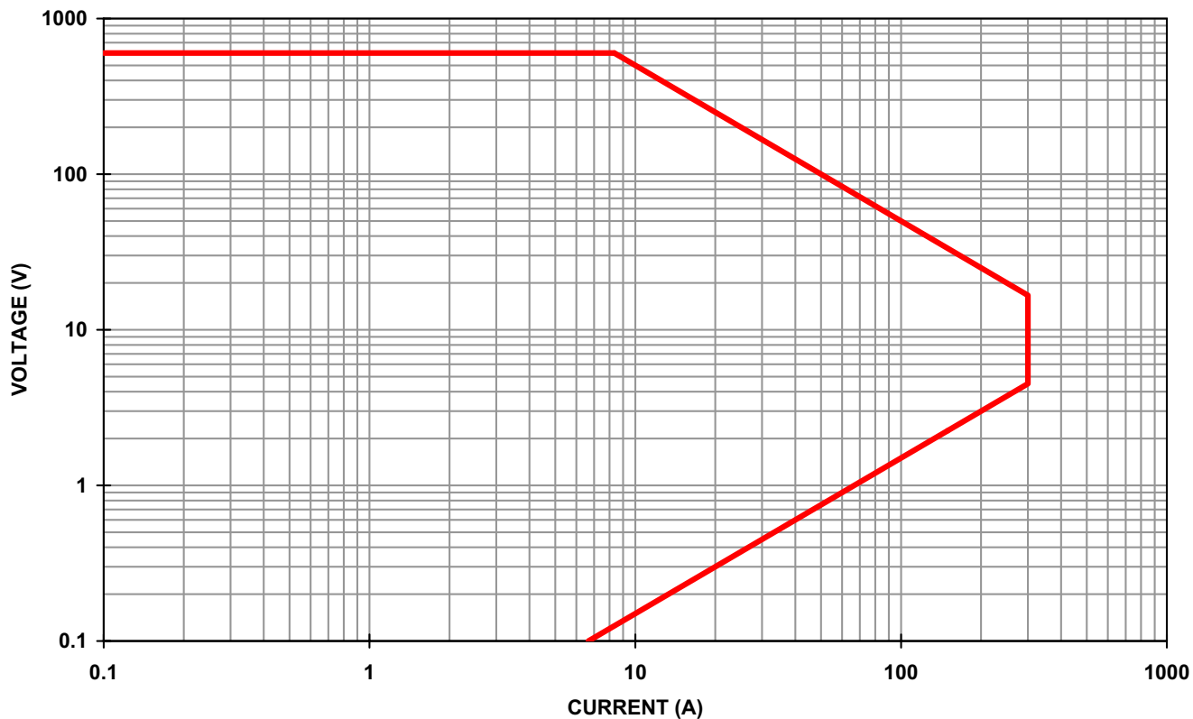
PLA5K-600-300 (600V,300A,5KW) OPERATIONAL CURVE
