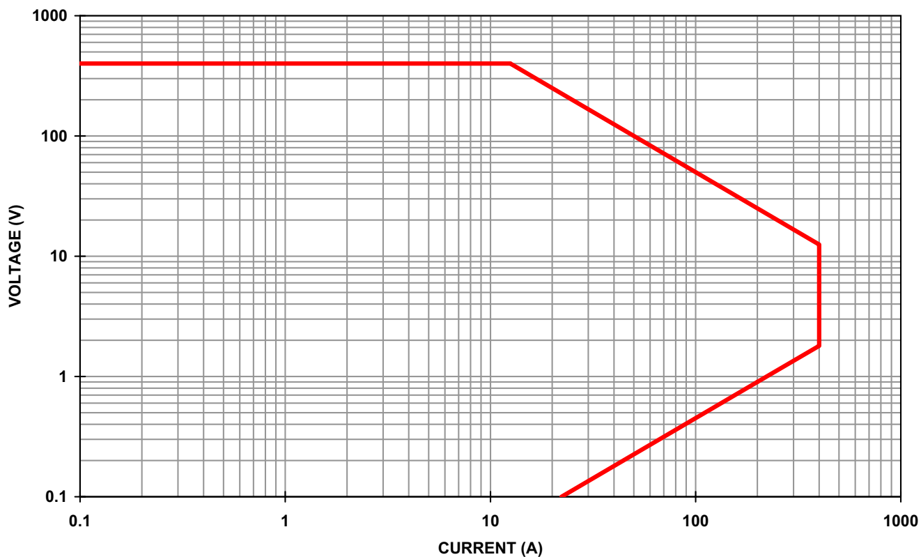
PLA5K-400-400 (400V,400A,5KW) OPERATIONAL CURVE
