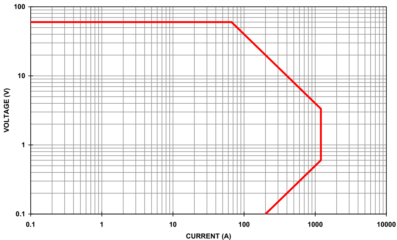
PLA4K-60-1200 (60V,1200A,4KW) OPERATIONAL CURVE
