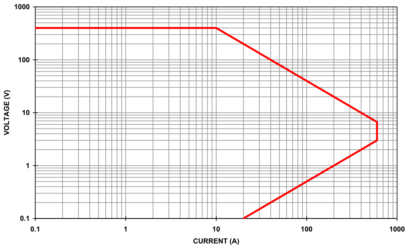
PLA4K-400-600 (400V,600A,4KW) OPERATIONAL CURVE
