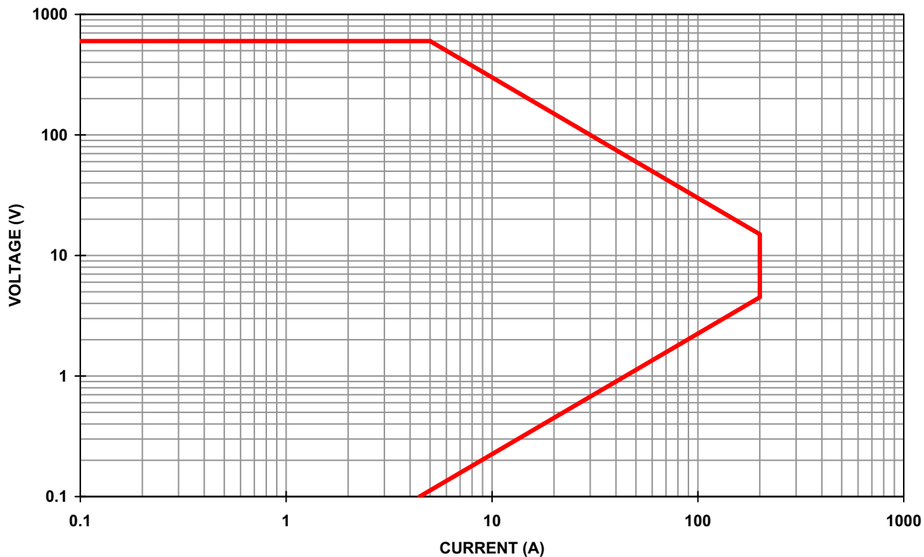
PLA3K-600-200 (600V,200A,3KW) OPERATIONAL CURVE
