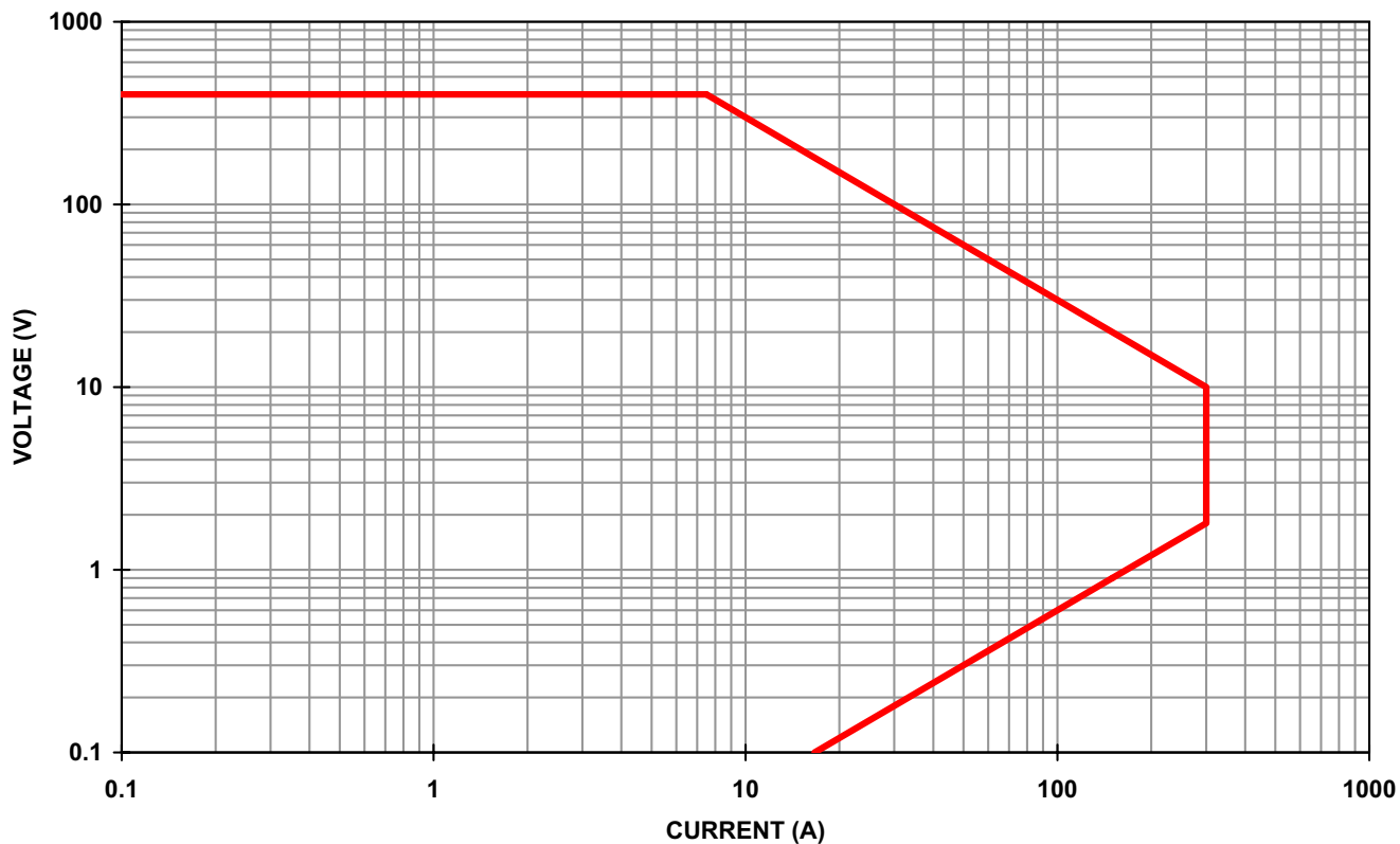
PLA3K-400-300 (400V,300A,3KW) OPERATIONAL CURVE
