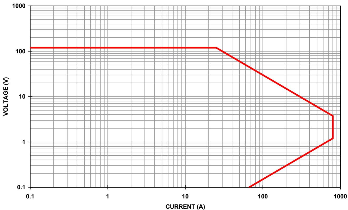
PLA3K-120-800 (120V,800A,3KW) OPERATIONAL CURVE
