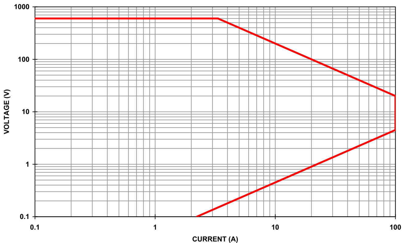
PLA2K-600-100 (600V,100A,2KW) OPERATIONAL CURVE
