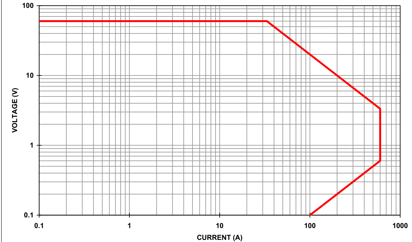
PLA2K-60-600 (60V,600A,2KW) OPERATIONAL CURVE
