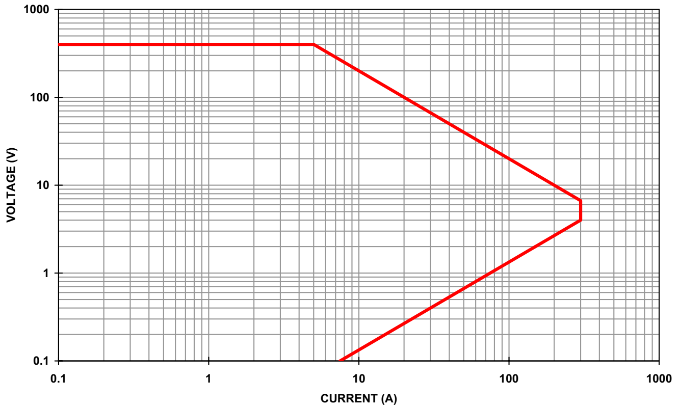
PLA2K-400-300 (400V,300A,2KW) OPERATIONAL CURVE
