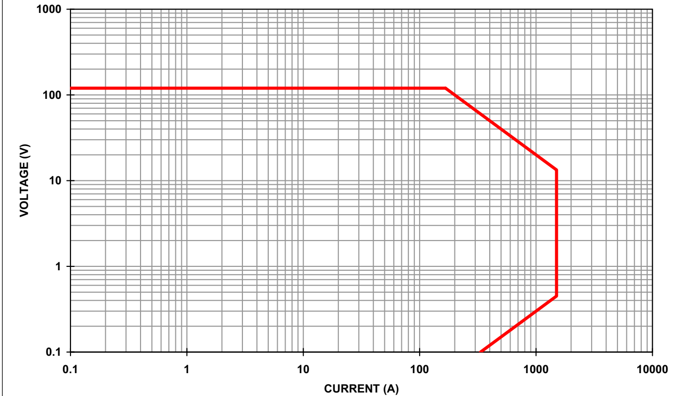
PLA20K-120-1500 (120V,1500A,20KW) OPERATIONAL CURVE
