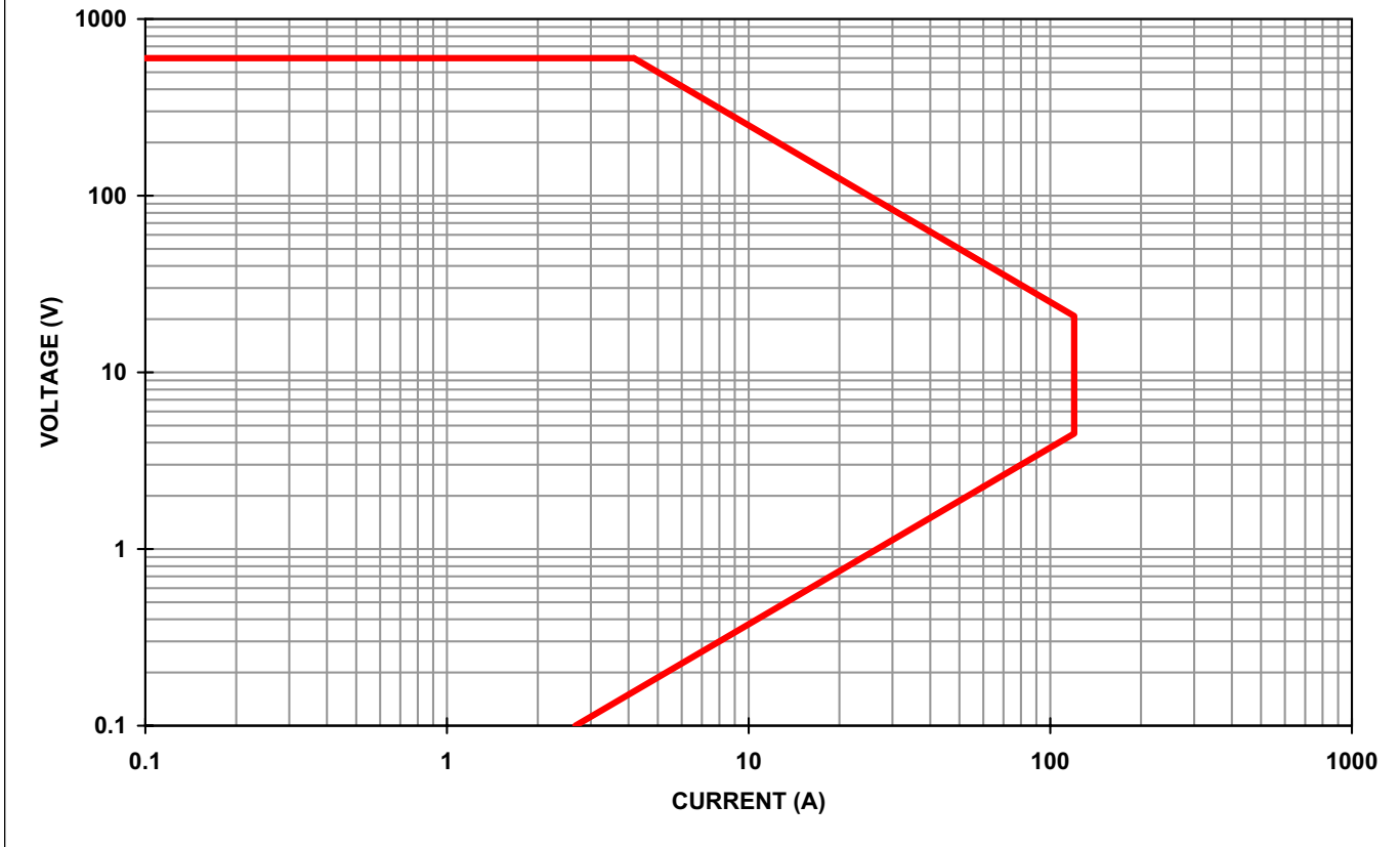
PLA2.5K-600-120 (600V,120A,2.5KW) OPERATIONAL CURVE
