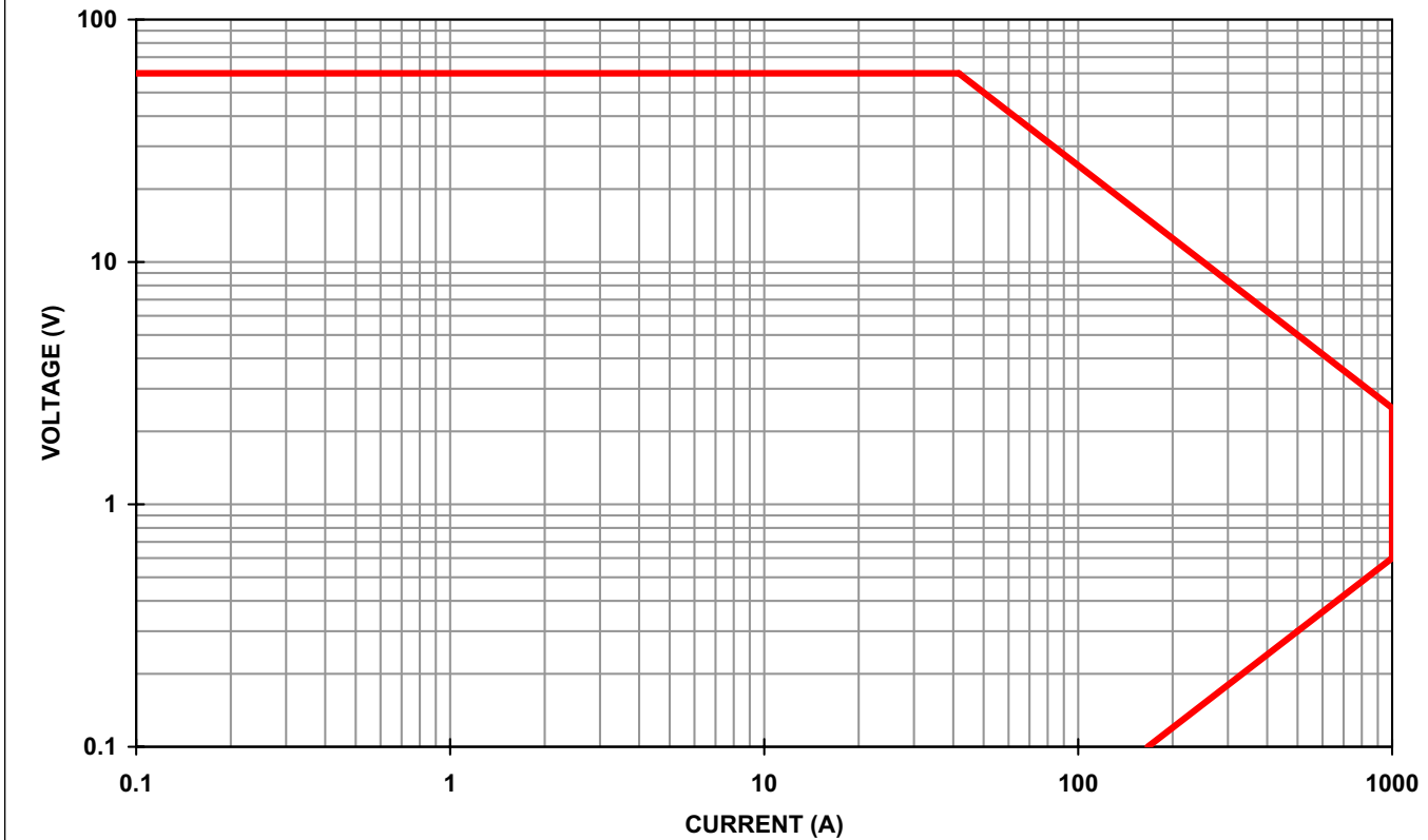
PLA2.5K-60-1000 (60V,1000A,2.5KW) OPERATIONAL CURVE
