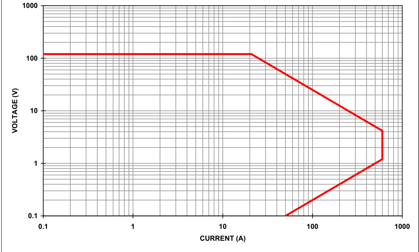
PLA2.5K-120-600 (120V,600A,2.5KW) OPERATIONAL CURVE
