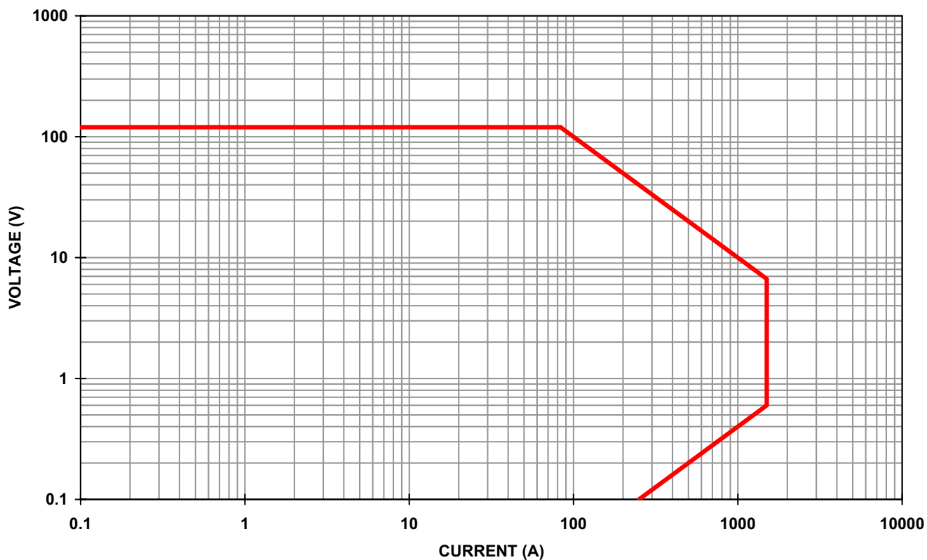
PLA10K-120-1500 (120V,1500A,10KW) OPERATIONAL CURVE
