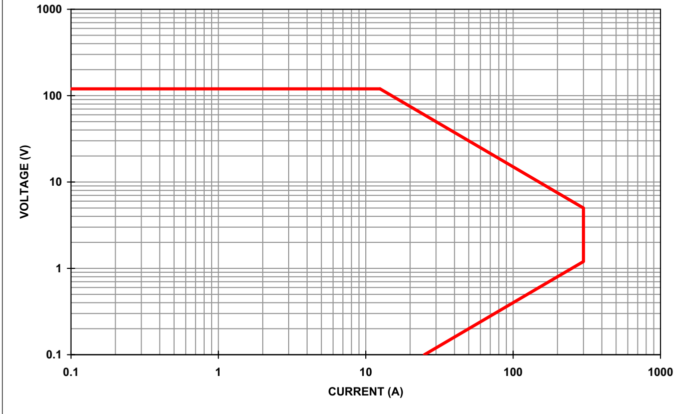
PLA1.5K-120-300 (120V,300A,1.5KW) OPERATIONAL CURVE
