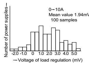
[Fig.-4] Distribution of Load Regulation (CV Characteristics)
