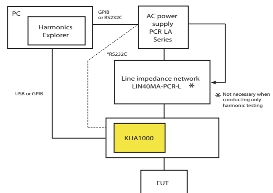
▲System configuration diagram for harmonic current and voltage fluctuation testing
