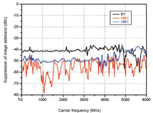
Measured suppression of image sideband
