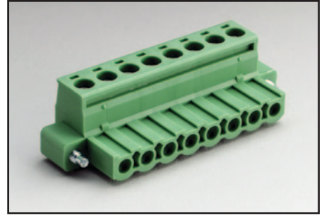
CS-846: Eight position connector with screw terminals or connection to test leads. For use with: 230X, 2510, 2510-AT
