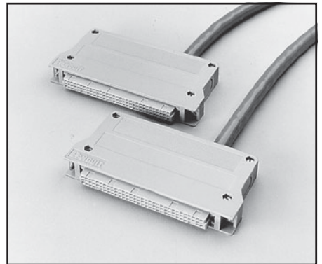
Model 7011-MTC-1: 1m (3.3 ft) mass terminated cable assembly for connection to 7011-C and other switching cards. The cable has 45 pairs with outer shield. The cable is terminated at each end with 96-pin female DIN connectors with strain relief. Also available in 2m (6.6 ft) length (Model 7011-MTC-2).
