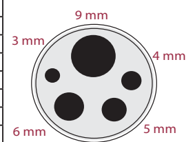
Multi-hole type 1 (CTC-320 A / 650 A)
