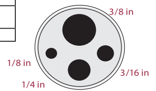
Multi-hole type 2 (CTC-320 A / 650 A)
