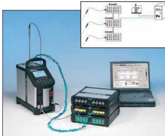
Picture 3: 2 ASM A models connected to the ASM B model, in order to obtain 24 channels. In this set-up the JOFRA ATC B model is used as a dry-block with the reference sensor connected to the reference input of the ATC. All controlled by JOFRACAL.
